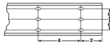
Bottom Mounting Holes, ½" x ⅜"
